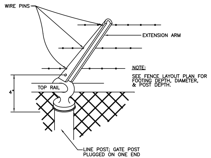
TYPICAL TOP RAIL GATE, END, & LINE POSTS NOT TO SCALE
