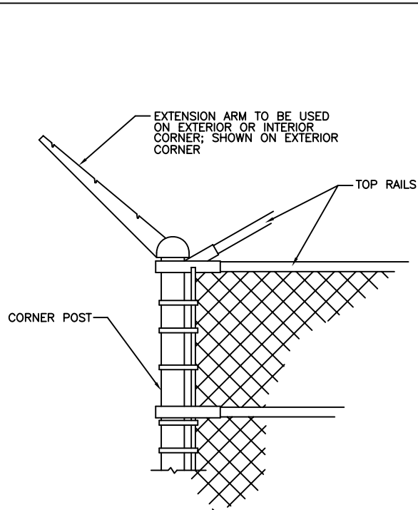
TYPICAL TOP RAIL CORNER & ANGLE POSTS NOT TO SCALE
