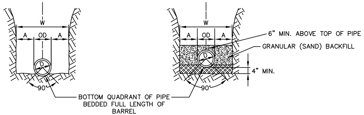
TRENCH IN EARTH
