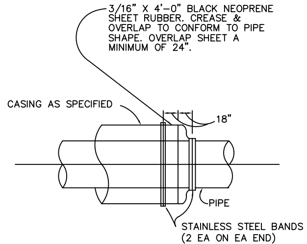
CASING END SEAL (TYPICAL EACH END)
